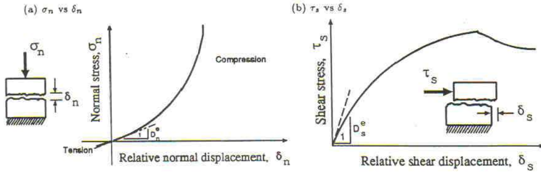
Figure 1 : Typical stress-relative displacement curve
