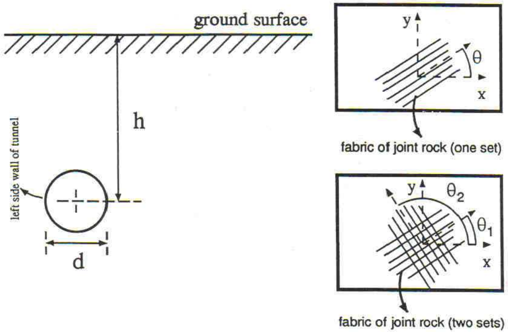
Figure 3 : Tunnel Geometry
